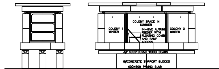
CROSS SECTION
