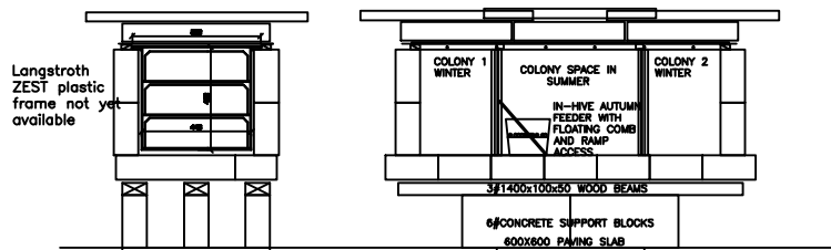
CROSS SECTION
